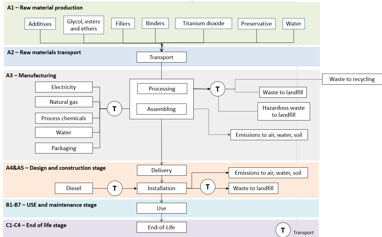
Figure 2: Flow Diagram for the MF Paints manufacturing process.
